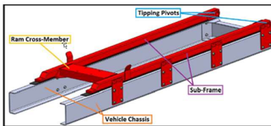
Figure 21- Basic Tipper Sub-Frame
