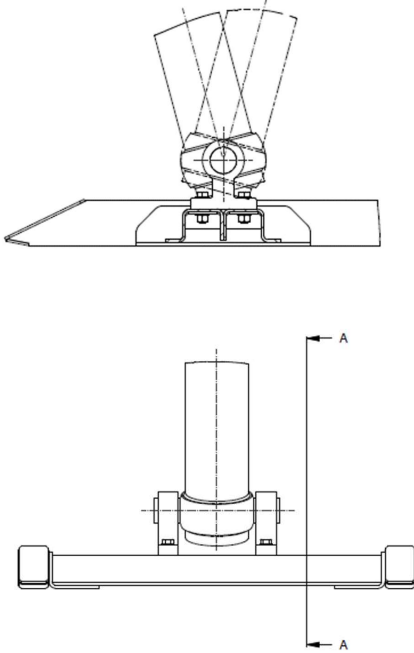
Figure 25 - Typical installation of the hoist cylinder.
