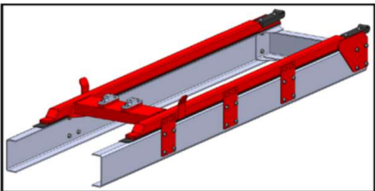
Figure 28 - Tipper sub-frame with integrated load cells
