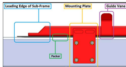
Figure 24 - Example of a suitable sub-frame leading edge, mounting Plate and Body guide (Guide Vane). Note additional examples in Modification code Section J (11)
